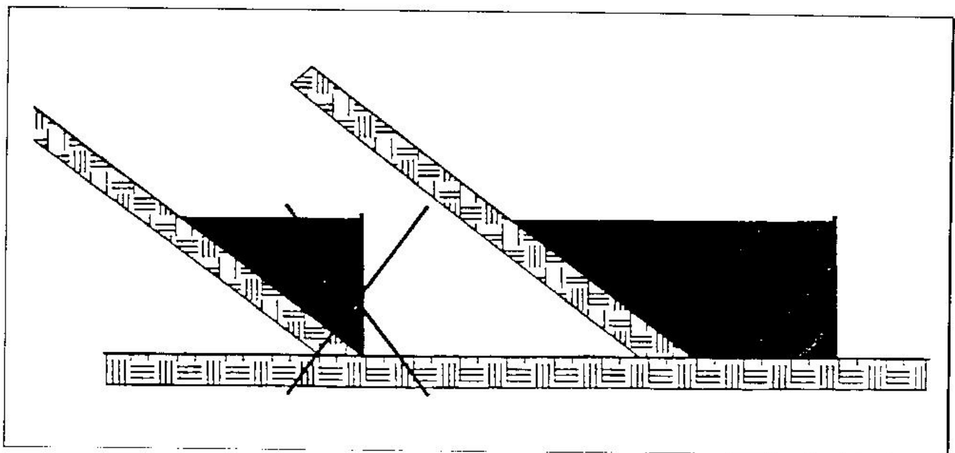
Proper Placement of a Silt Fence at the Toe of a Slope
