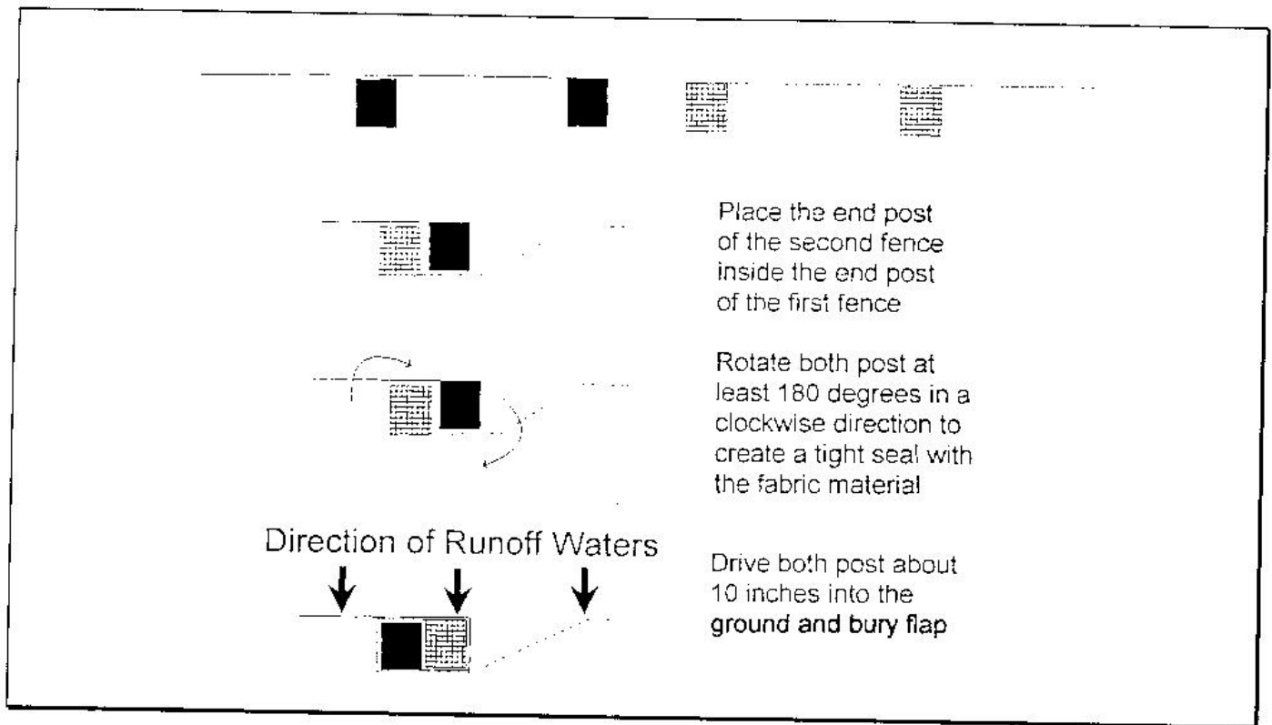
Attaching Two Silt Fences
